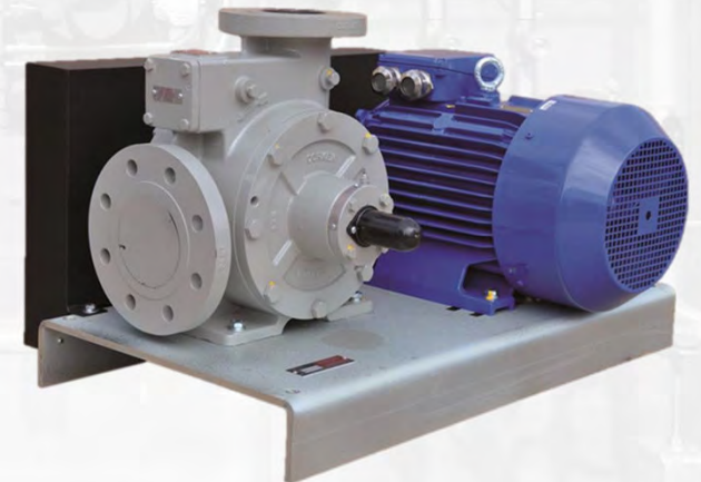
▶ Pump unit Z4500 with V-belt drive
