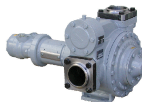
pump unit with hydraulic motor
