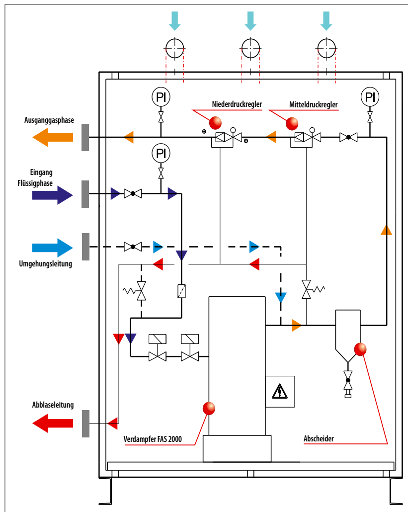
Typical diagram of vaporizer unit FAS 2000
