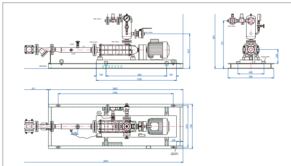
Dimensional drawing of complete suction pump unit capacity 50/100 l/min with 3-phase motors 5/6,8 kW
