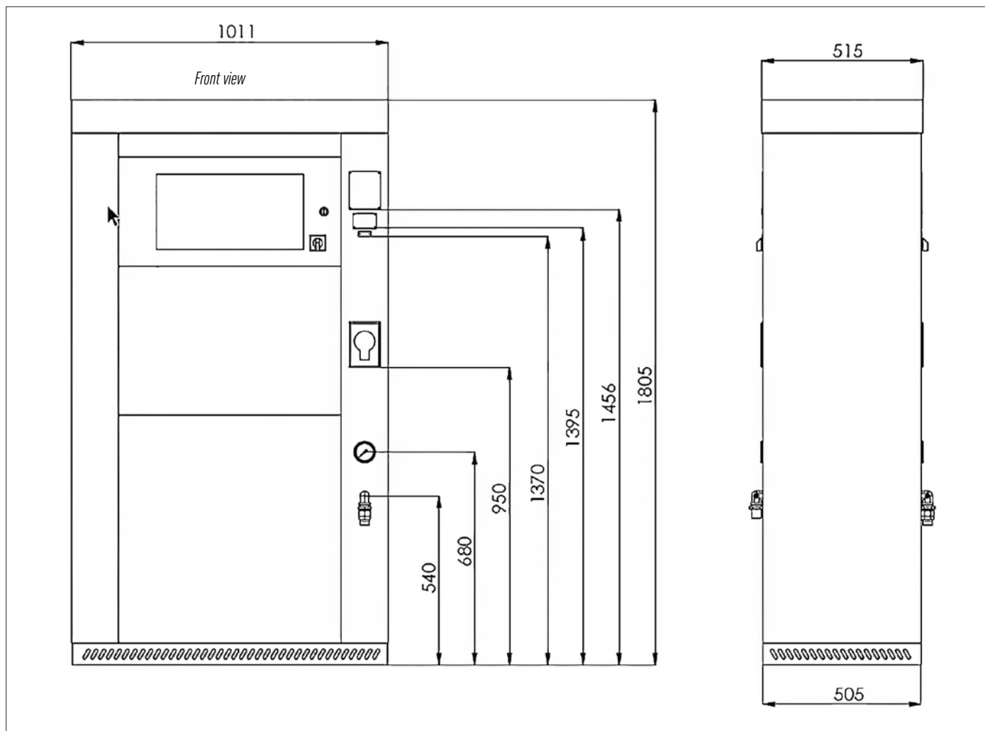
Dimensional drawing of electronic LPG-dispenser
