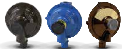
SECOND STAGE REGULATOR LV3403 SERIES LV4403 SERIES LV5503 SERIES
